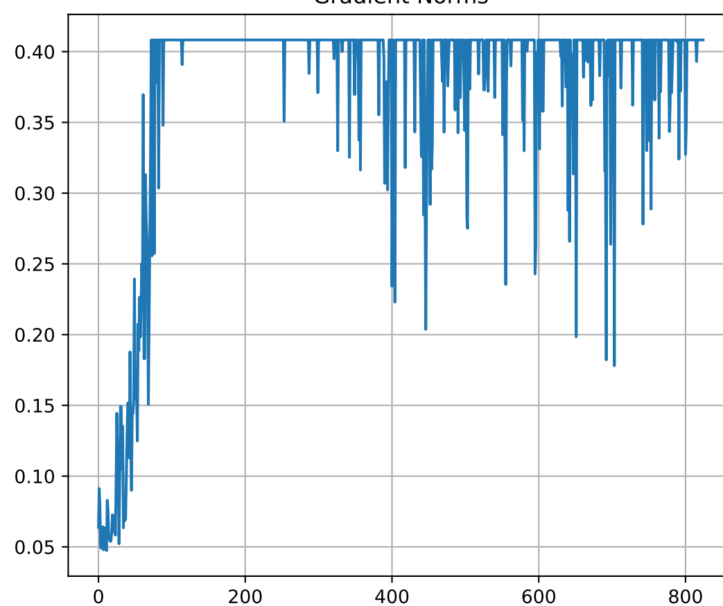
Evaluation Metrics
