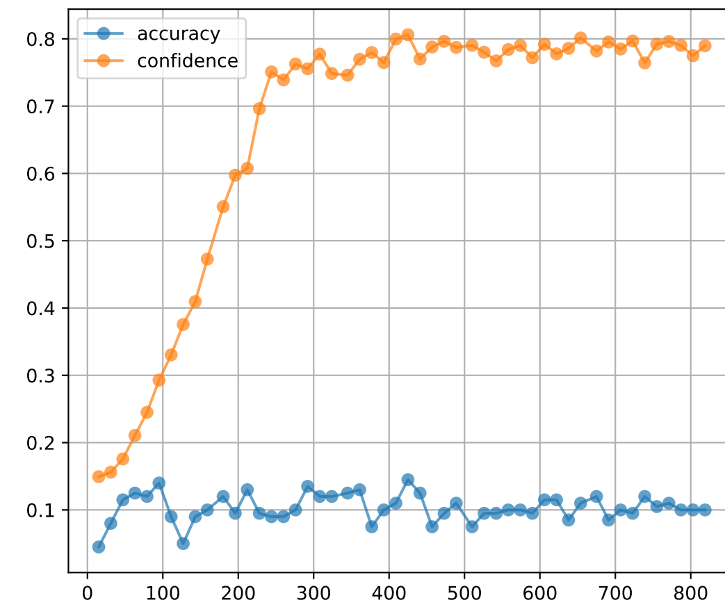
Evaluation Metrics
